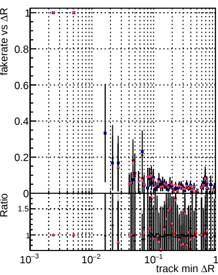
Fake rate vs \Delta R(\text{track, jet}) for trainOldFiles125_v2_prelimWPM_epoch4, trainOldFiles125_v2_prelimWPM_epoch4, trainOldFiles125_v2_ANDLessRetrain_epoch4, and trainOldFiles125_v2_prelimWPM_epoch4
