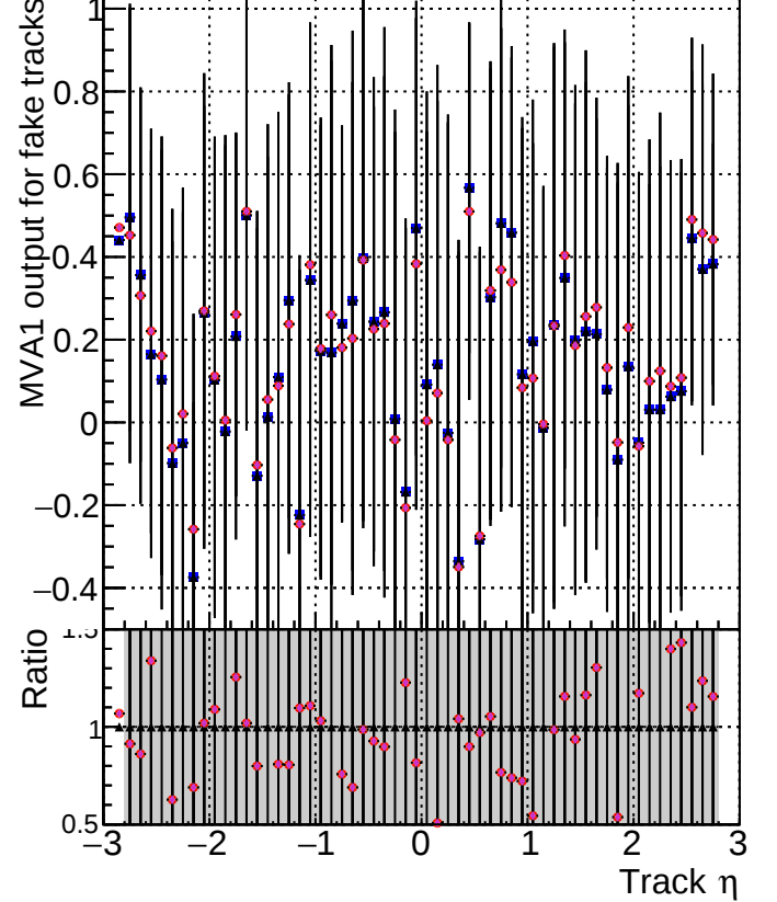
MVA1 of associated tracks (recoToSim) vs. track \eta Legend: Blue star: DQM_mkFit5_XiMinusNOPU_base Red diamond: DQM_mkFit5_XiMinusNOPU_retrainOldFiles125_v2_prelimWPM_epoch4 Black triangle: DQM_mkFit6_XiMinusNOPU_base Black circle: DQM_mkFit6_XiMinusNOPU_retrainOldFiles125_v2_prelimWPM_epoch4 Purple star: DQM_mkFit5_XiMinusNOPU_retrainOldFiles125_v2_ANDPLessRetrain_epoch4
