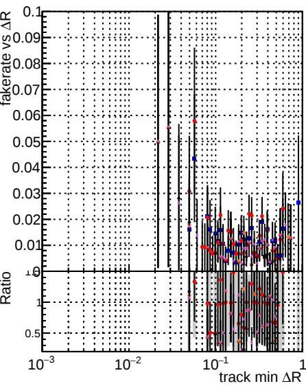
Fake rate vs \Delta R(\text{track, jet}) for RetrainOldFiles125_v2_prelimWPM_epoch4 and RetrainOldFiles125_v2_ANDLessRetrain_epoch4
