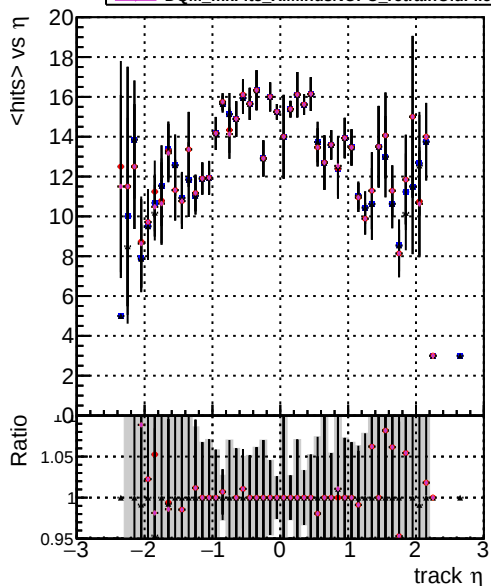
mean hits vs \eta Legend: DOM mkFit5 XMinusNOPU_retrainOldFiles125_v2_prelimWPM_epoch4 (blue), DOM mkFit5 XMinusNOPU_base (red), DOM mkFit5 XMinusNOPU_retrainOldFiles125_v2_prelimWPM_epoch4 (orange), DOM mkFit5 XMinusNOPU_retrainOldFiles125_v2_ANDPLeRetrain_epoch4 (purple)
