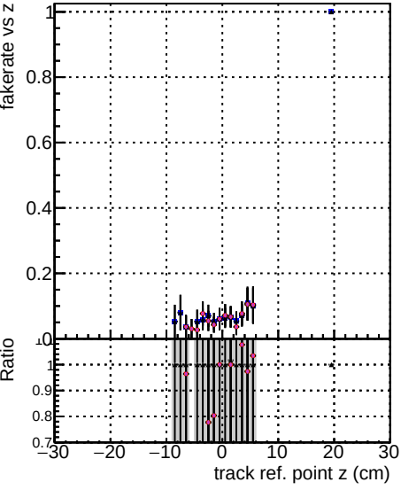
Fake rate vs v DOM mkFI15 xMinisNOPI base trainOldFiles125 v2 prelimWPM epoch4 DOM mkFI15 xMinisNOPI base trainOldFiles125 v2 ANDLessRetran epoch4
