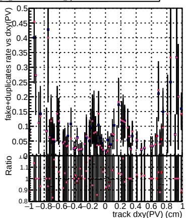
y2_prelimWPM_epoch4 y2_ANDPLessRetrain_epoch4
