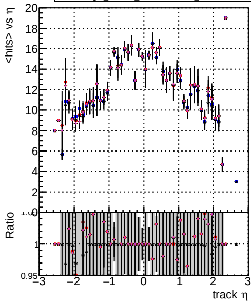
mean hits DOM mkFit5 XMinusNOPU_retrainOldFiles125_v2_prelimWPM_epoch4 DOM mkFit5 XMinusNOPU_base DOM mkFit6 XMinusNOPU_retrainOldFiles125_v2_prelimWPM_epoch4 DOM mkFit5 XMinusNOPU_retrainOldFiles125_v2_ANDPLessRetrain_epoch4
