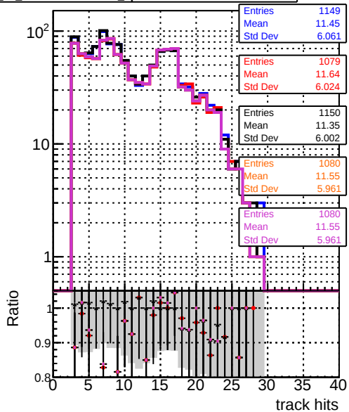
mean hits DOM mkFit5 XMinusNOPU_retrainOldFiles125_v2_prelimWPM_epoch4 DOM mkFit5 XMinusNOPU_base DOM mkFit6 XMinusNOPU_retrainOldFiles125_v2_prelimWPM_epoch4 DOM mkFit5 XMinusNOPU_retrainOldFiles125_v2_ANDPLessRetrain_epoch4
