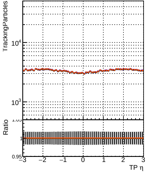
N of simulated tracks vs \eta Legend: DQM_mkFit5_XiMinusNOPU_base DQM_mkFit5_XiMinusNOPU_retrainOldFiles125_v2_prelimWPM_epoch4 DQM_mkFit6_XiMinusNOPU_base DQM_mkFit6_XiMinusNOPU_retrainOldFiles125_v2_prelimWPM_epoch4
