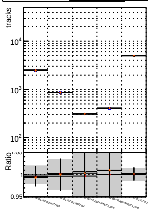
N of reco track vs. \chi^2 for different datasets and methods
