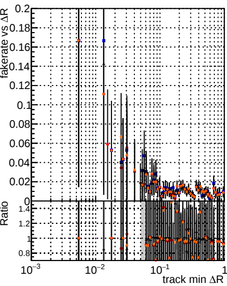
Fake rate vs \Delta R(\text{track, jet}) base retrainOldFiles125_v2_prelimWPM_epoch4 base retrainOldFiles125_v2_prelimWPM_epoch4
