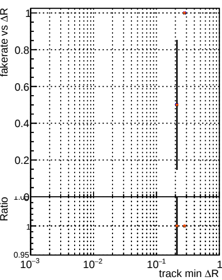
Fake rate vs \Delta R(\text{track, jet}) DQM mkFit5 xMinusNOPI base retainOldFiles125_v2_prelimWPM_epoch4 DQM mkFit6 xMinusNOPI base retainOldFiles125_v2_prelimWPM_epoch4 DQM mkFit6 xMinusNOPI base retainOldFiles125_v2_prelimWPM_epoch4
