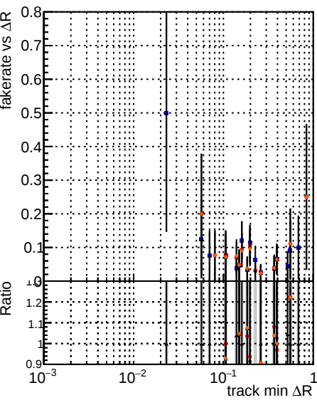
Fake rate vs ΔR(track, jet) for various models and datasets. The legend indicates: DOM mkFit5 (blue), DOM mkFit6 (red), DOM mkFit12 (orange), XMinus (black), and base (grey). The datasets are: retainOldFiles125_v2_prelimWPM_epoch4 and base.
