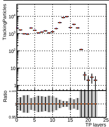
N of sim —●— DQM_mkFit6_XiMinusNO
