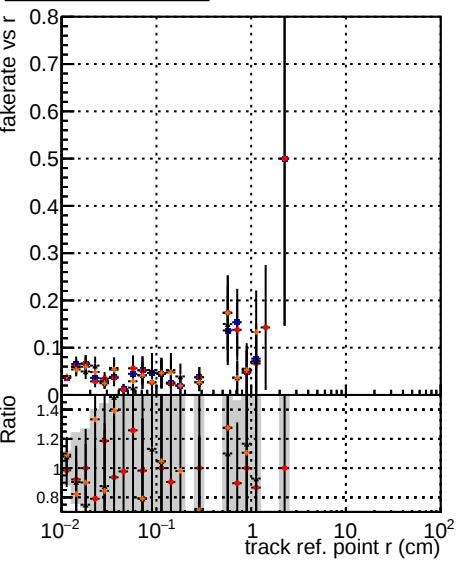
Fake rate vs v DOM mkFit5 XMinus NOPI base DOM mkFit6 XMinus NOPI base DOM mkFit12 XMinus NOPI base DOM mkFit16 XMinus NOPI base retrainOldFiles125_v2_prelimWPM_epoch4 retrainOldFiles125_v2_prelimWPM_epoch4
