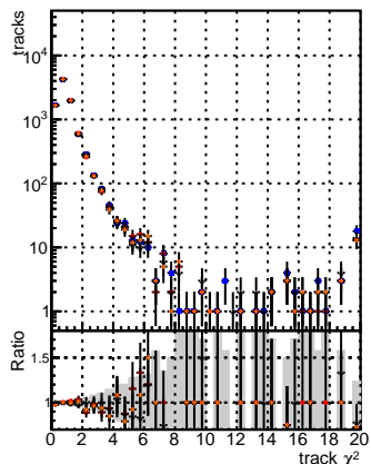
N of reco track vs. \chi^2 for BGM, BGM+H15, BGM+H15+XIM, BGM+H15+XIM+NOPI, BGM+H15+XIM+NOPI+recoOldFiles125_v2_prelimWPM_epoch4, BGM+H15+XIM+NOPI+recoOldFiles125_v2_prelimWPM_epoch4
