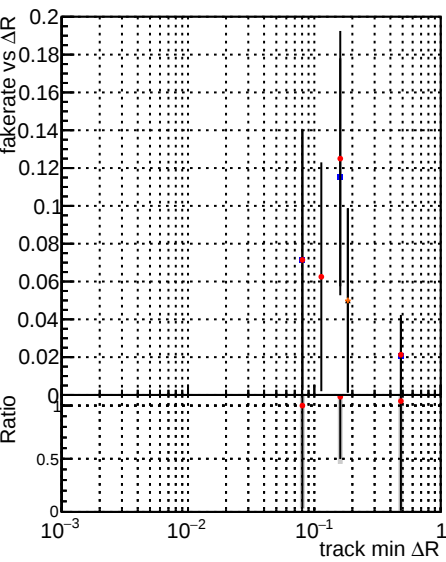
Fake rate vs \Delta R(\text{track, jet}) for base, retainOldFiles125_v2_prelimWPM_epoch4, and retrainOldFiles125_v2_prelimWPM_epoch4 models. Legend: DOM (black), mkrF15 (blue), mkrF16 (red), XMinus (orange).
