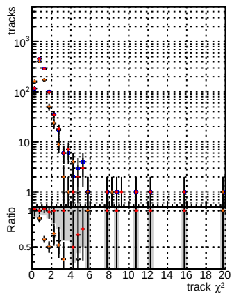
N of reco track vs. \chi^2 for BSM, SM, and NLO. Legend: BSM (blue), SM (red), NLO (orange), and NLO (black). Data is from trainOldFiles125_v2_prelimWPM_epoch4 and trainOldFiles125_v2_prelimWPM_epoch4.
