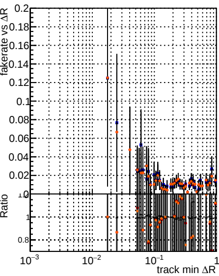
Fake rate vs \Delta R(\text{track, jet}) for base, retrainOldFiles125_v2_prelimWPM_epoch4, and retrainOldFiles125_v2_prelimWPM_epoch4 models. Legend: DOM (black), mkrF15 (blue), mkrF16 (orange), XiMinus (red).
