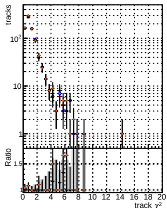
N of reco track vs. \chi^2 for different models and datasets. Legend: BSM (black), mF15 (blue), mF16 (orange), XIMINUS (red). Datasets: trainOldFiles125 v2_prelimWPM_epoch4, trainOldFiles125 v2_prelimWPM_epoch4, trainOldFiles125 v2_prelimWPM_epoch4.
