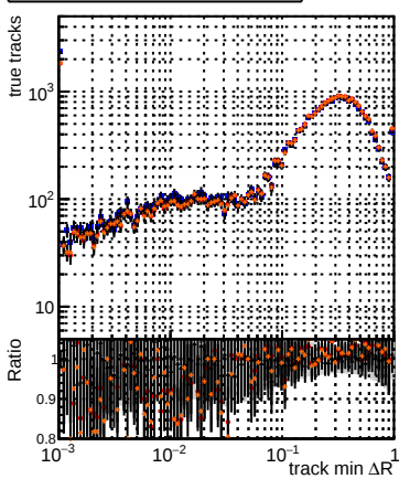
N of associated tracks (recoToSim) vs dR
