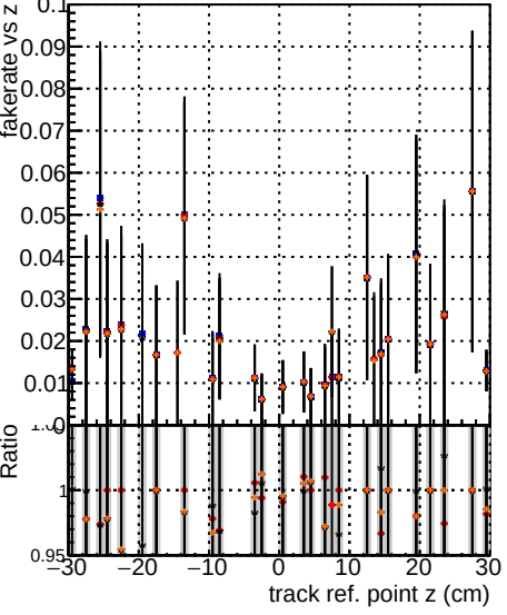
Fake rate vs v DOM mkrF15 XMinuS NOPI base DOM mkrF16 XMinuS NOPI base DOM mkrF16 XMinuS NOPI base retrainOldFiles125 v2 prelimWPM epoch4 retrainOldFiles125 v2 prelimWPM epoch4
