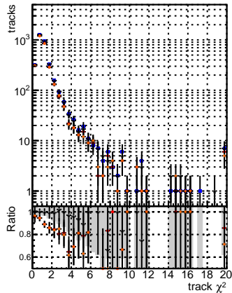
N of reco track vs. \chi^2 for \chi^2 bins: 0-1, 1-2, 2-3, 3-4, 4-5, 5-6, 6-7, 7-8, 8-9, 9-10, 10-11, 11-12, 12-13, 13-14, 14-15, 15-16, 16-17, 17-18, 18-19, 19-20
