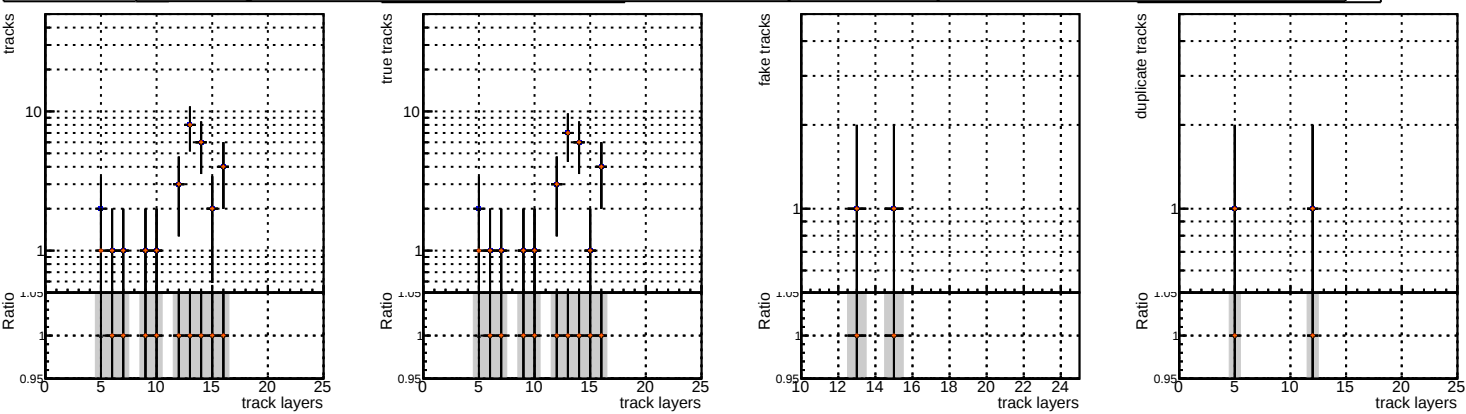
Legend: DOM, mkr, hit5, xim, minus, NOPU, base, retrainOldFiles125_v2_prelimWPM_epoch4, mkr, hit6, xim, minus, NOPU, base, retrainOldFiles125_v2_prelimWPM_epoch4, 3 layer
