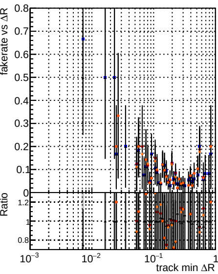
Fake rate vs \Delta R(\text{track, jet}) | Duplicates Rate vs \Delta R(\text{track, jet}) | Pileup rate vs \Delta R(\text{track, jet}) Legend: DOM (black), mkrF15 (blue), mkrF16 (orange), XMinus (red), base (grey), retainOldFiles125_v2_prelimWPM_epoch4 (green), base (grey), retainOldFiles125_v2_prelimWPM_epoch4 (green).
