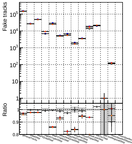
Number ● DQM mkFit6 XiMinusPU base ● DQM mkFit6 XiMinusPU retrainOldFiles125_v2_prelimWPM_epoch4
