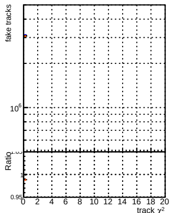
N of associated (recoToSim) fake tracks vs. \chi^2 for various datasets and models.
