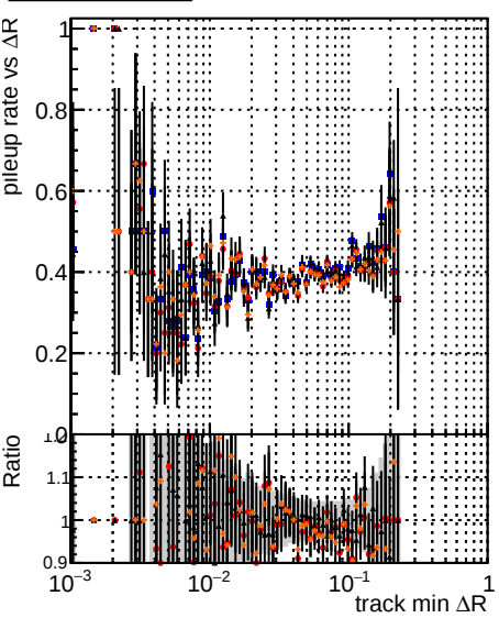
DOM mkFit5 XiMinusPU base DOM mkFit6 XiMinusPU base DOM mkFit12 XiMinusPU base DOM mkFit16 XiMinusPU base retrainOldFiles125 v2_prelimWPM_epoch4 base retrainOldFiles125 v2_prelimWPM_epoch4
