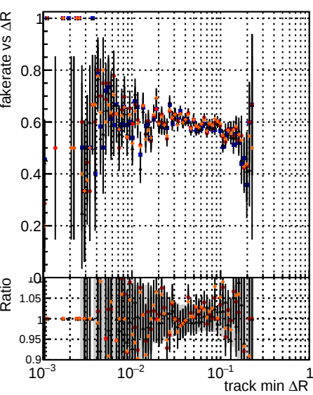
DOM mkFit5 XiMinusPU base DOM mkFit6 XiMinusPU base DOM mkFit12 XiMinusPU base DOM mkFit16 XiMinusPU base retrainOldFiles125 v2_prelimWPM_epoch4 base retrainOldFiles125 v2_prelimWPM_epoch4
