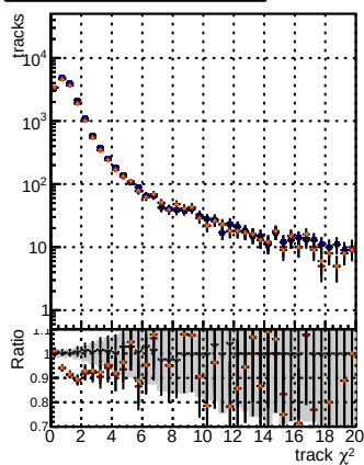
N of reco track vs. \chi^2 for \chi^2 bins: [0, 2], (2, 4], (4, 6], (6, 8], (8, 10], (10, 12], (12, 14], (14, 16], (16, 18], (18, 20]
