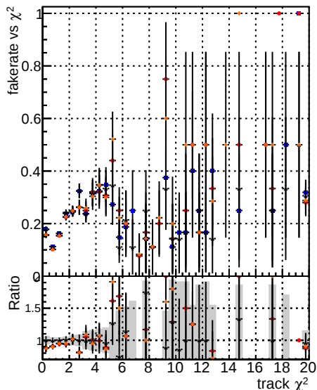
Fake rate vs. BQM mkr fit5 XIM MinusPU base trainOldFiles125_v2_prelimWPM_epoch4 trainOldFiles125_v2_prelimWPM_epoch4
