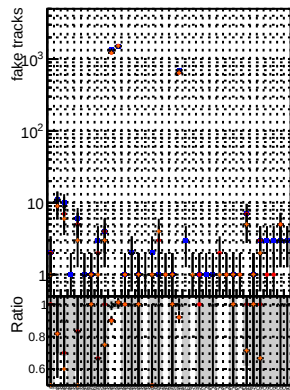
N of associated (recoToSim) fake tracks vs. \chi^2
