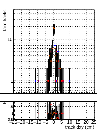
N of associated (recoToSim) looper tracks vs dxy
