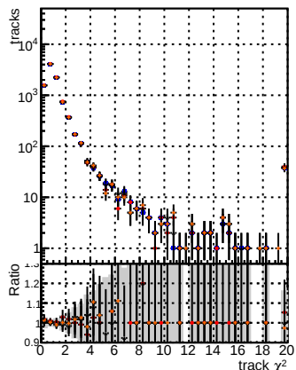
N of reco track vs. \chi^2 for various models and baselines.
