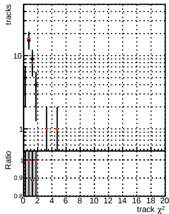
N of reco track vs. \chi^2 for different track counts and normalized \chi^2 bins. Legend: \chi^2 bins (0-1, 1-2, 2-3, 3-4, 4-5, 5-6, 6-7, 7-8, 8-9, 9-10, 10-11, 11-12, 12-13, 13-14, 14-15, 15-16, 16-17, 17-18, 18-19, 19-20) and track counts (1, 2, 3, 4, 5, 6, 7, 8, 9, 10, 11, 12, 13, 14, 15, 16, 17, 18, 19, 20).
