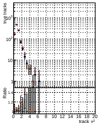
N of reco track vs. \chi^2 for BSM, mF15, XIMINUS, BSM base, RainOldFiles125_v2_prelimWPM_epoch4
