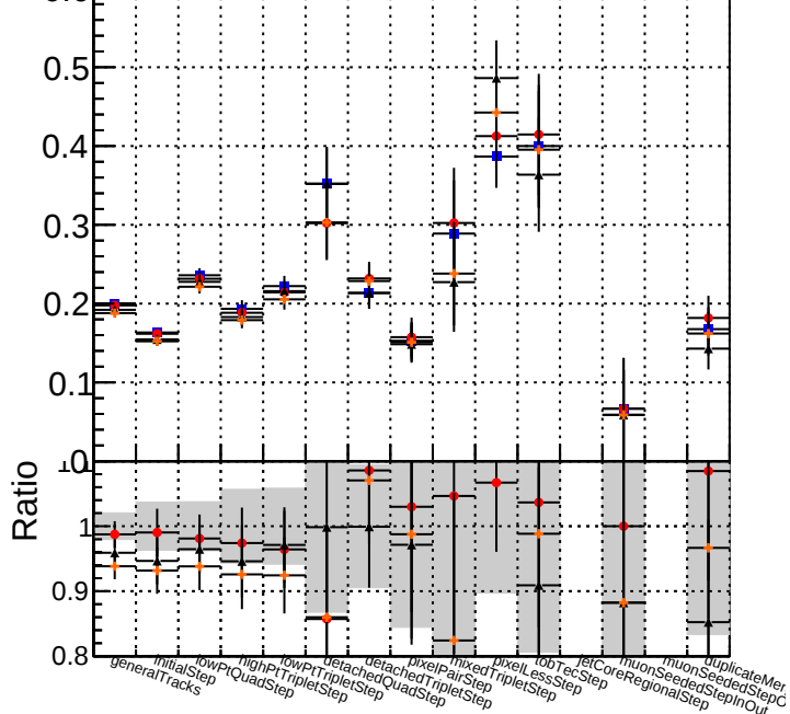
Pileup rate vs collection
