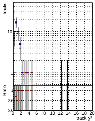
N of reco track vs. \chi^2 for DGM mF16 XMinUS base trainOldFiles125_v2_prelimWPM_epoch4
