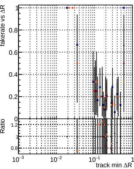
Fake rate vs \Delta R(\text{track, jet}) for various models and datasets.
