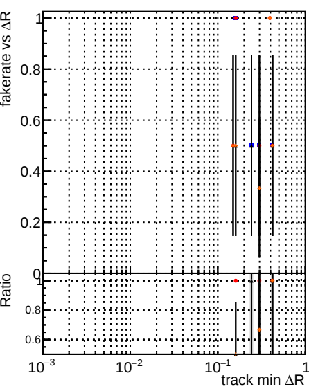
Fake rate vs \Delta R(\text{track, jet}) for base, retrainOldFiles125_v2_prelimWPM_epoch4, and xiMinusPU models.
