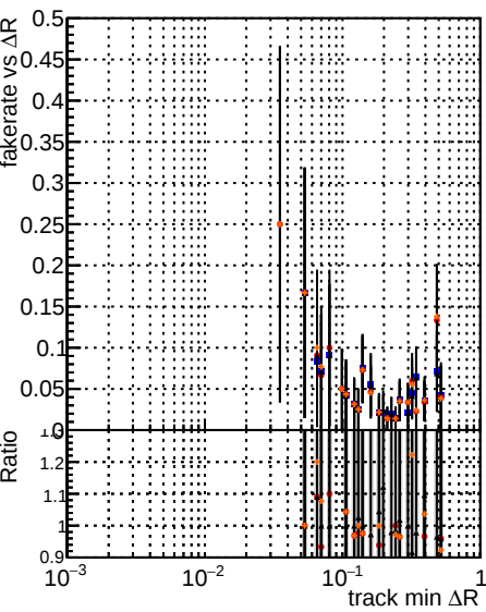
Fake rate vs ΔR(track, jet) DOM mkrF15 XiMinusPU base retrainOldFiles125_v2_prelimWPM_epoch4
