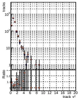
N of reco track vs. \chi^2 for BSM, mFIS, XIMINUS, XIMINUS+PH, BSM+OldFiles125_v2_prelimWPM_epoch4, BSM+OldFiles125_v2_prelimWPM_epoch4, BSM+OldFiles125_v2_prelimWPM_epoch4, BSM+OldFiles125_v2_prelimWPM_epoch4
