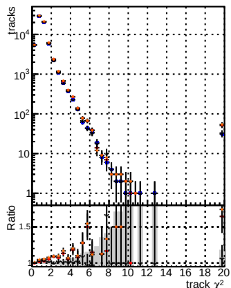
N of reco track vs. \chi^2 for BSM, mF15, mF16, mF17, mF18, mF19, mF20, mF21, mF22, mF23, mF24, mF25, mF26, mF27, mF28, mF29, mF30, mF31, mF32, mF33, mF34, mF35, mF36, mF37, mF38, mF39, mF40, mF41, mF42, mF43, mF44, mF45, mF46, mF47, mF48, mF49, mF50, retainOldFiles125_v2_prelimWPM_epoch4
