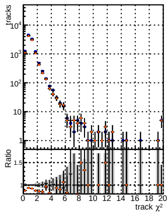
N of reco track vs. \chi^2 for different models: DGM, mF16, mF15, mF14, mF13, mF12, mF11, mF10, mF9, mF8, mF7, mF6, mF5, mF4, mF3, mF2, mF1, mF0, mF-1, mF-2, mF-3, mF-4, mF-5, mF-6, mF-7, mF-8, mF-9, mF-10, mF-11, mF-12, mF-13, mF-14, mF-15, mF-16, mF-17, mF-18, mF-19, mF-20, mF-21, mF-22, mF-23, mF-24, mF-25, mF-26, mF-27, mF-28, mF-29, mF-30, mF-31, mF-32, mF-33, mF-34, mF-35, mF-36, mF-37, mF-38, mF-39, mF-40, mF-41, mF-42, mF-43, mF-44, mF-45, mF-46, mF-47, mF-48, mF-49, mF-50.
