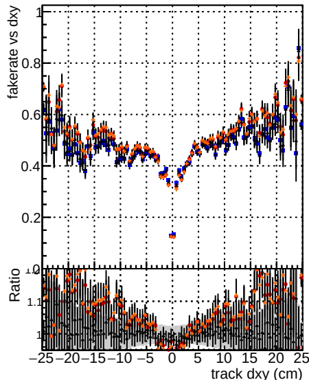
BQM mkt fit5 XIM fit10 XIM fit20 XIM PU TrainOldFiles125_v2_prelimWPM_epoch4 TrainOldFiles125_v2_prelimWPM_epoch4
