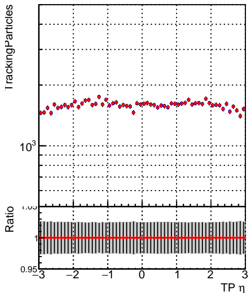
—•— DQM_mkFit5_TTbase —•— DQM_mkFit5_TT_retrainOldFiles125_v2_prelimWP_epoch4
