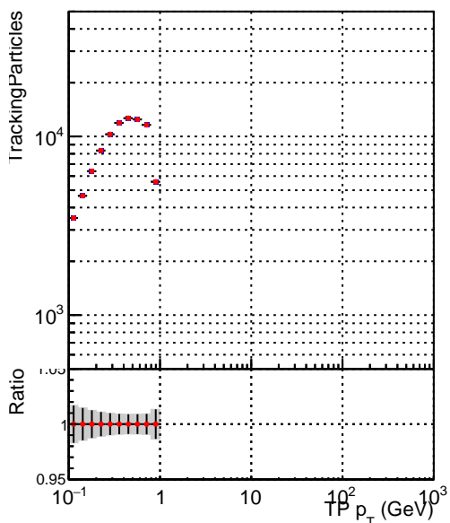
—•— DQM_mkFit5_TTbase —•— DQM_mkFit5_TT_retrainOldFiles125_v2_prelimWP_epoch4
