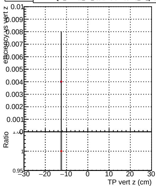
Efficiency — DQM_mkFit5_TT_retrainOldFiles125_v2_prelimWP_epoch4
