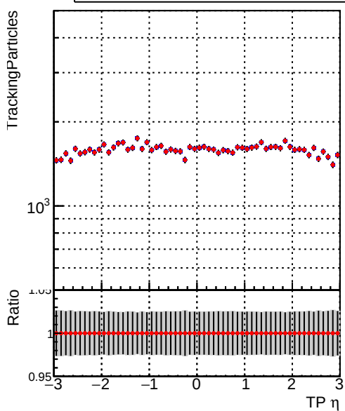
N of simulated tracks vs \eta Legend: - \blacksquare DQM_mkFit_TTbase - \bullet DQM_mkFit5_TT_retrainOldFiles125_v2_prelimWP_epoch4
