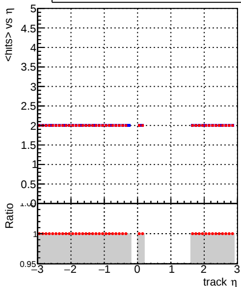
mean hit — DQM_mkFit5_TTbase — DQM_mkFit5_TT_retrainOldFiles125_v2_prelimWP_epoch4
