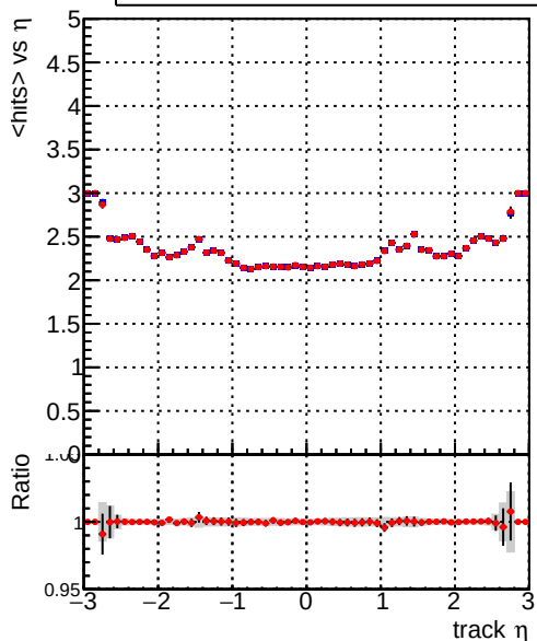
mean hits vs \eta — DQM_mkFit_TTbase — DQM_mkFit5_TT_retrainOldFiles125_v2_prelimWP_epoch4
