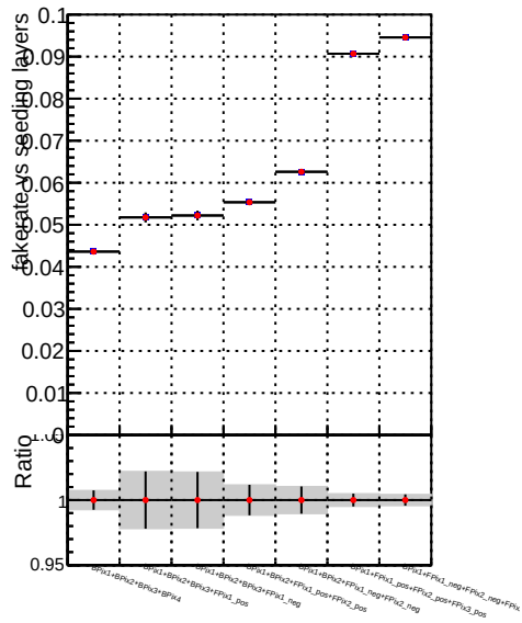
Fake rate vs. DQM_mkFit5_TTbase DQM_mkFit5_TT_retrainOldFiles125_v2_prelimWP_epoch4
