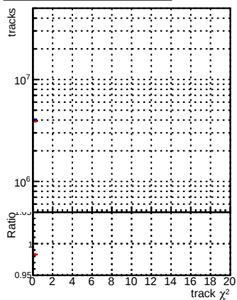
N of reco track vs. \chi^2 for DQM_mkFit_TTbase and DQM_mkFit5_TT_retrainOldFiles125_v2_prelimWP_epoch4
